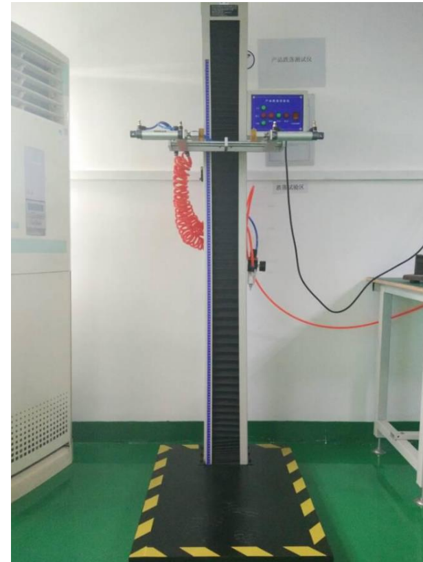
Drop Tester
