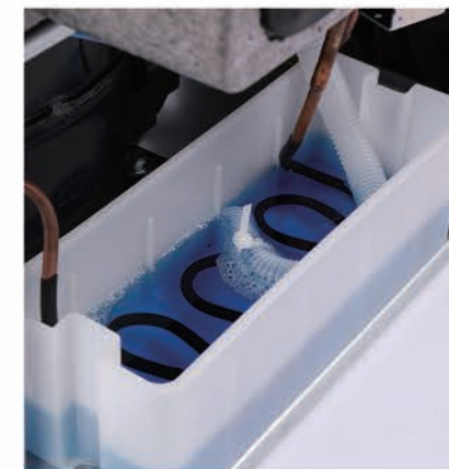
操作台化霜水自蒸发系统 Self-evaporating system of console defrosted water 不需蒸发包和排水管。 No need for evaporation packs and drains.
