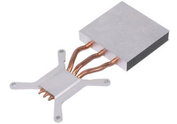
Stacked fins heat sink with heat pipes
