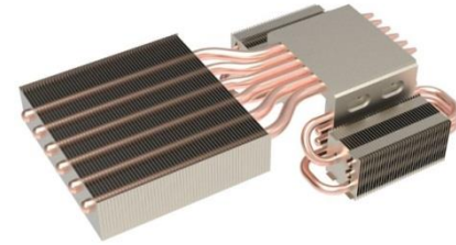
Stacked fins heat sink with heat pipes
