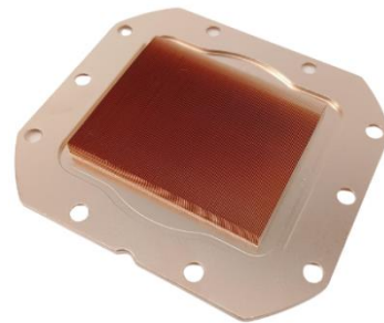
Skived copper plate
