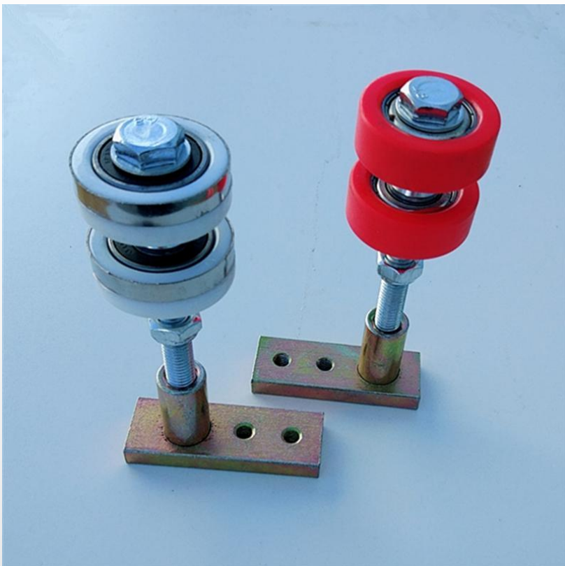
定制异型件/酒店宴会厅使用 Customized non-standard parts/for hotel banquet halls
