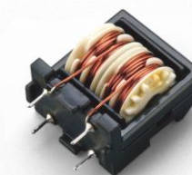
Common mode inductor
