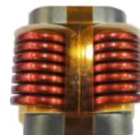
Single-phase common mode inductor
