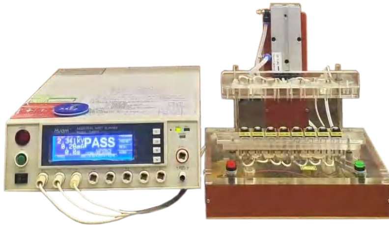
八通道自動高壓測試儀 Auto Hipot tester with eight lines
