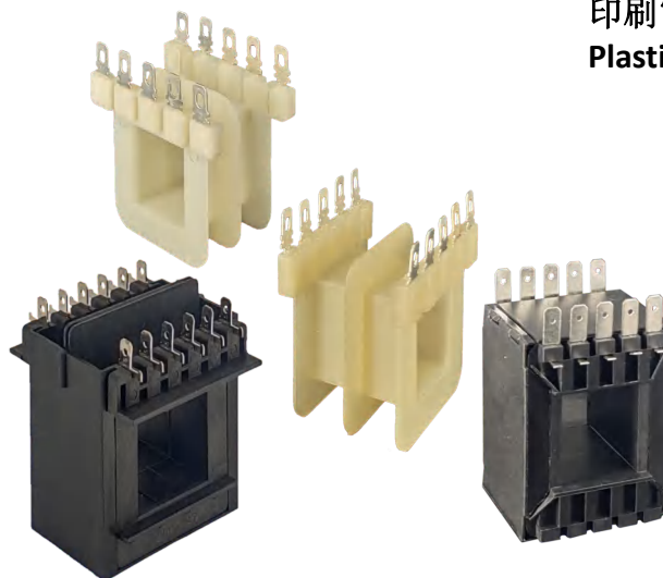
快速連接端子連接方式塑膠骨架 Plastic bobbins with quick connection terminals
