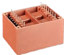
灌封變壓器塑膠骨架 Plastic bobbins for encapsulated transformers
