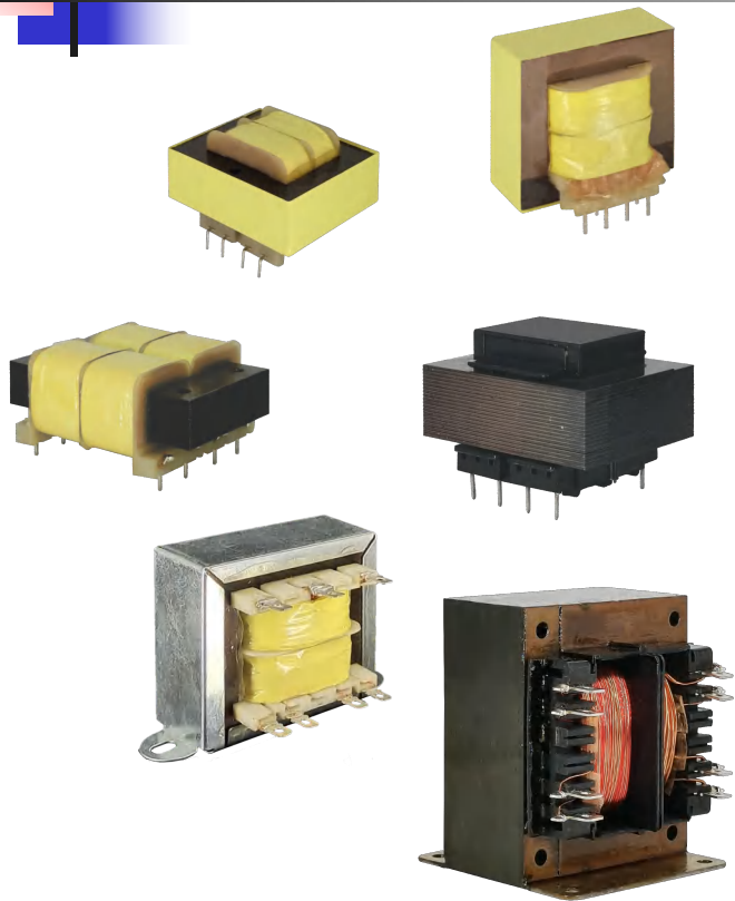
印刷電路板安裝和快速連接的低頻電源變壓器 PCB mounted and fast connected low frequency power transformers
