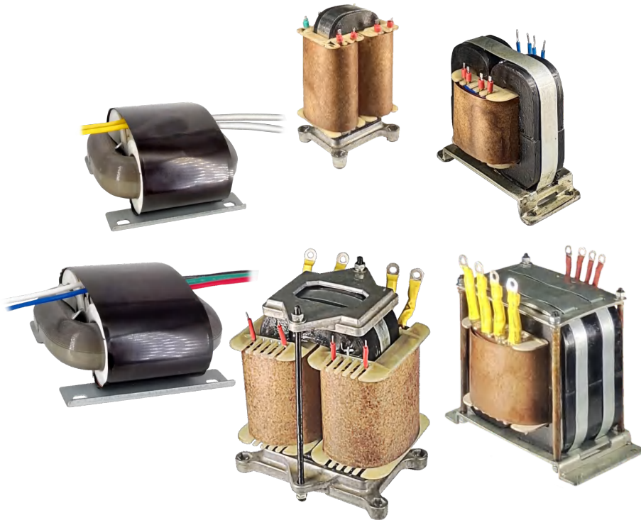
特殊類型電源變壓器(R, CD, ED型等) Special type power transformers (R, CD, ED etc.)
