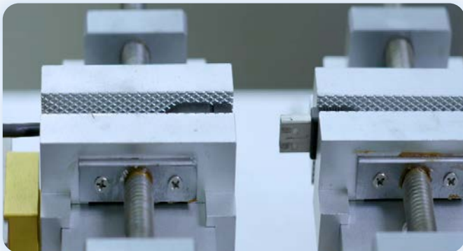
Pull force test
