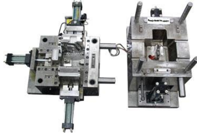
Two color injection mould
