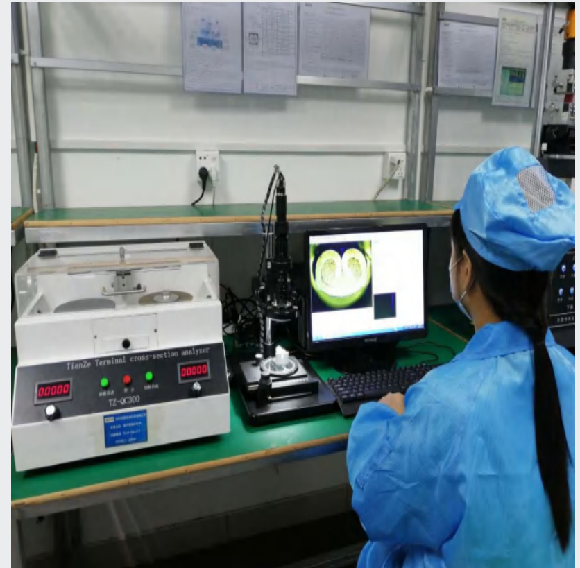
◆ Terminal Cross -section analyzer of crimping terminal ◆ 端子截面分析仪
