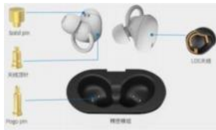
TWS earphone
