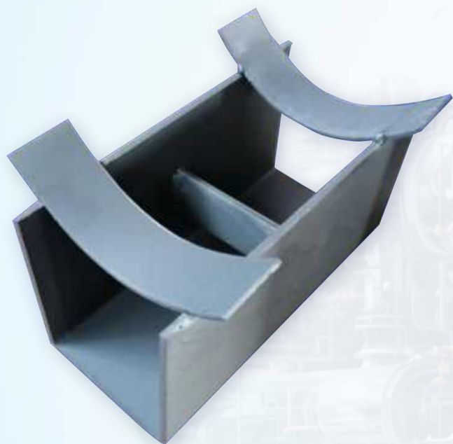
曲面槽滑动支座 Curved groove sliding support
