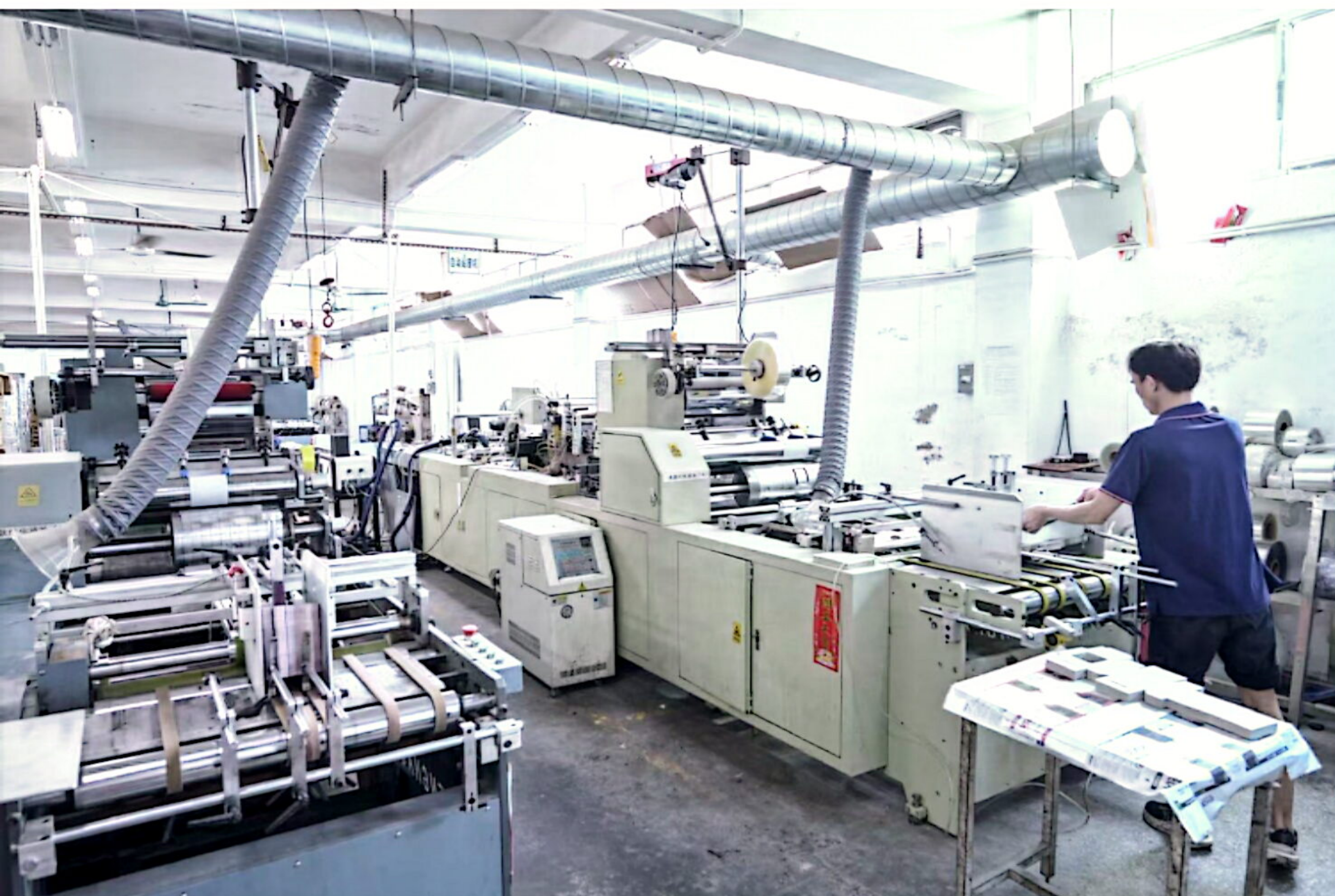
Full-automatic window patching machine
