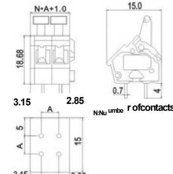
KF188
