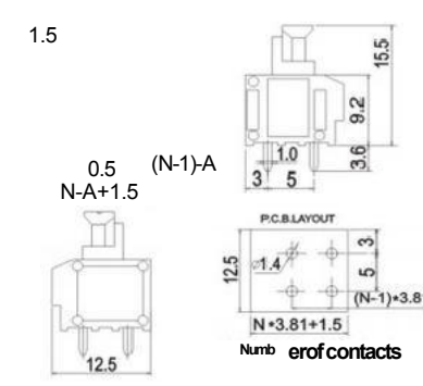
KF124B
