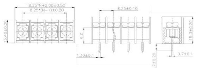
KF30C KF30CM
