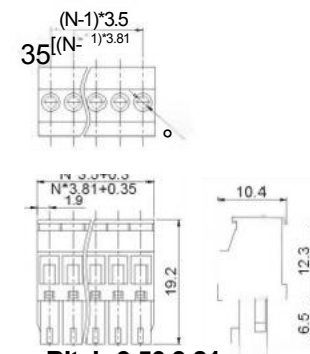
KF2EDGK-3.5 KF2EDGK-3.81
