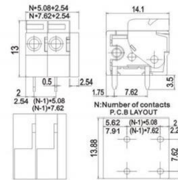
KF142R
