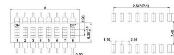
KF1027-C
