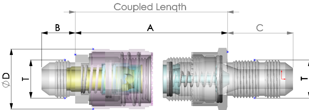
阴接头 Coupling
