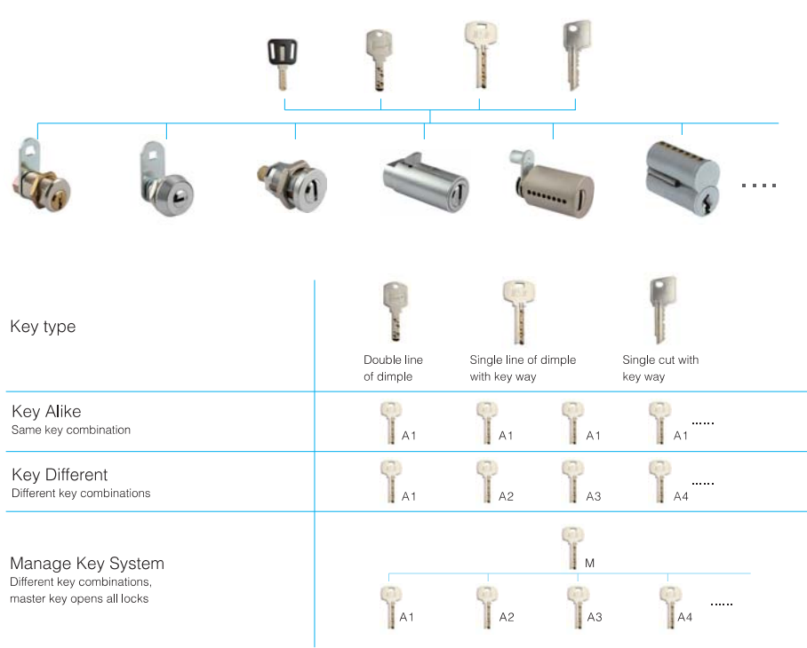
Dimple Key System Applicable For Different Locks
