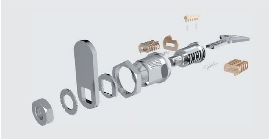
M3-Lock System Applicable For Different Locks
