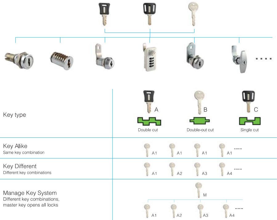
Laser Key System Applicable For Different Locks
