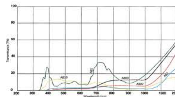
Neutral Density Filter 中性滤光片
