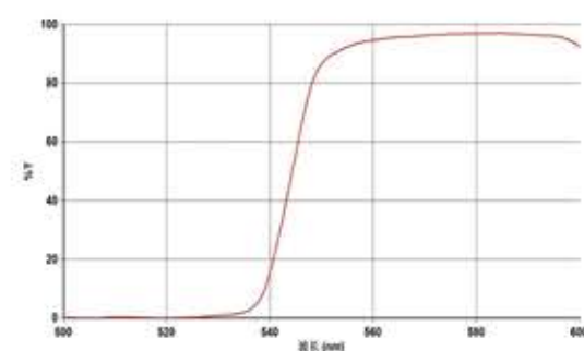
Longpass Filter 长通滤光片
