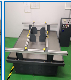
Simulated transport vibration platform
