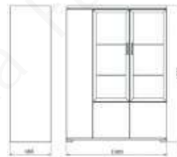
酒柜 Wine cabinet H1775*W1300*D465mm
