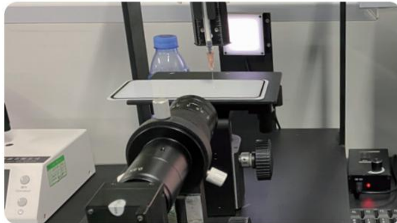
Water Drop Angle Test ▲
