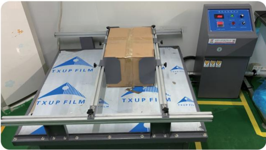
▲ Reliability Test
