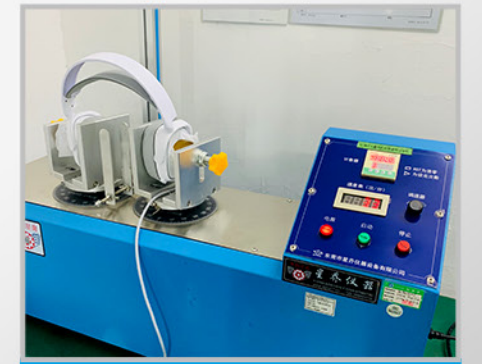
Headset Waving Strength Tester
