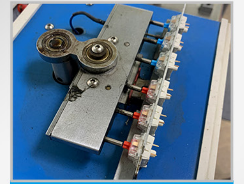
Switches Clicking Life Tester
