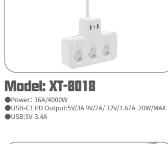
Model: XT-8018 ●Power: 16A/4000W ●USB-C1 PD Output:5V/3A 9V/2A/ 12V/1.67A 20W/MAX ●USB-V-3.4A
