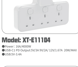
Model: XT-E11104 ●Power: 16A/4000W ●USB-C1 PD Output:5V/3A 9V/2A/ 12V/1.67A 20W/MAX ●USB-V-3.4A
