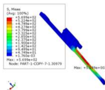
Terminal Stress Analysis
