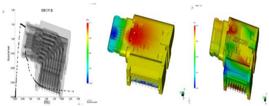
Mold flow analysis
