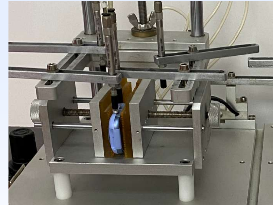
Through hundreds of thousands of consecutive clicks Test button durability
