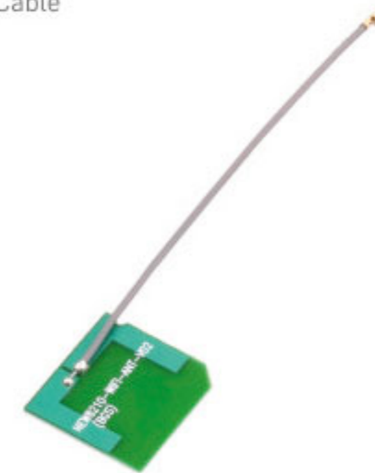
Bluetooth Antenna Long Range WiFi Antenna Cable I-PEX MHF 20278-001R-13 to PCB RF1.13 Cable
