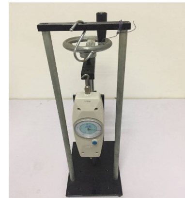
Pull Testing
