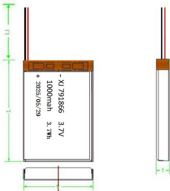
(Maximum) Dimension: T×W×L: 7.9mm×18.0mm×68.0mm Battery
