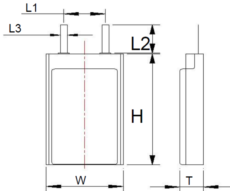
(Maximum) Dimension: T×W×H: 7.9mm×18.0mm×66.0mm Cell
