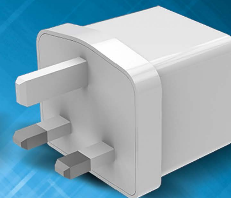
USB Type-C™ wall charger (WAC340SF-A) • Input: 90-240V AC • Output: 5V/3.4A with USB Type-C and USB Type-A ports • Various plugs available
