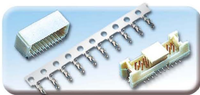
Wire-to-board crimp connectors Pitch: 0.9-8.0mm
