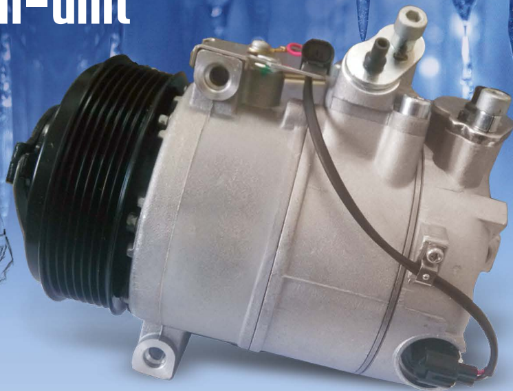
A/C compressor (SE6/7PW-6/7SEU) • Externally controlled variable swashplate type • Suitable for Mercedes-Benz, Audi, BMW and Toyota vehicles • Replacement for 6/7SEU series compressors
