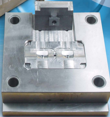
Injection mold for plastic/LSR parts
