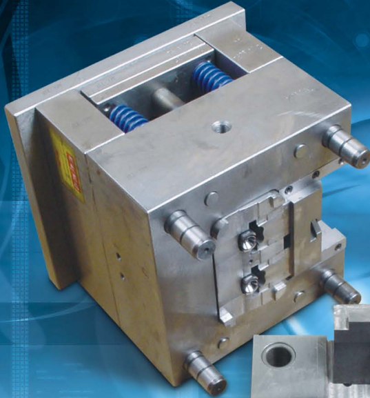
Injection mold for plastic/LSR parts
